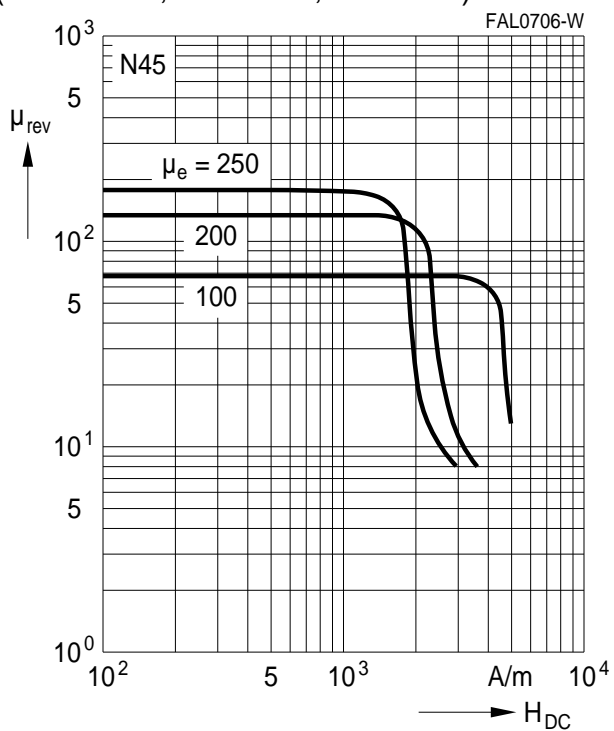
DC magnetic bias of P and RM cores (typical values) ( \dot{B} \leq 0.25 \text{ mT} , f = 10 \text{ kHz} , T = 25 \text{ }^\circ\text{C} )
